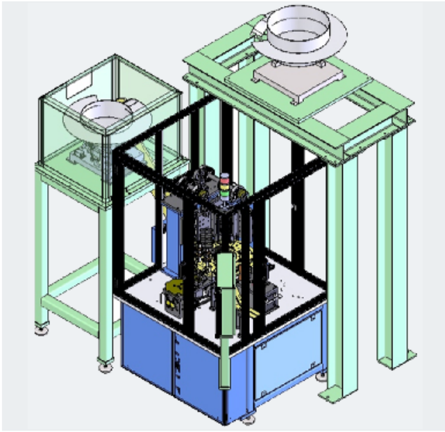
Priming Machines
